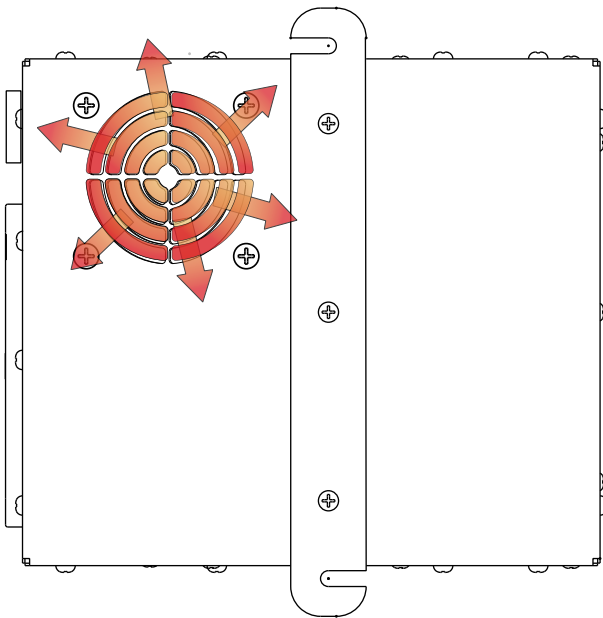
Figure 2.6.1 Top Outlet
