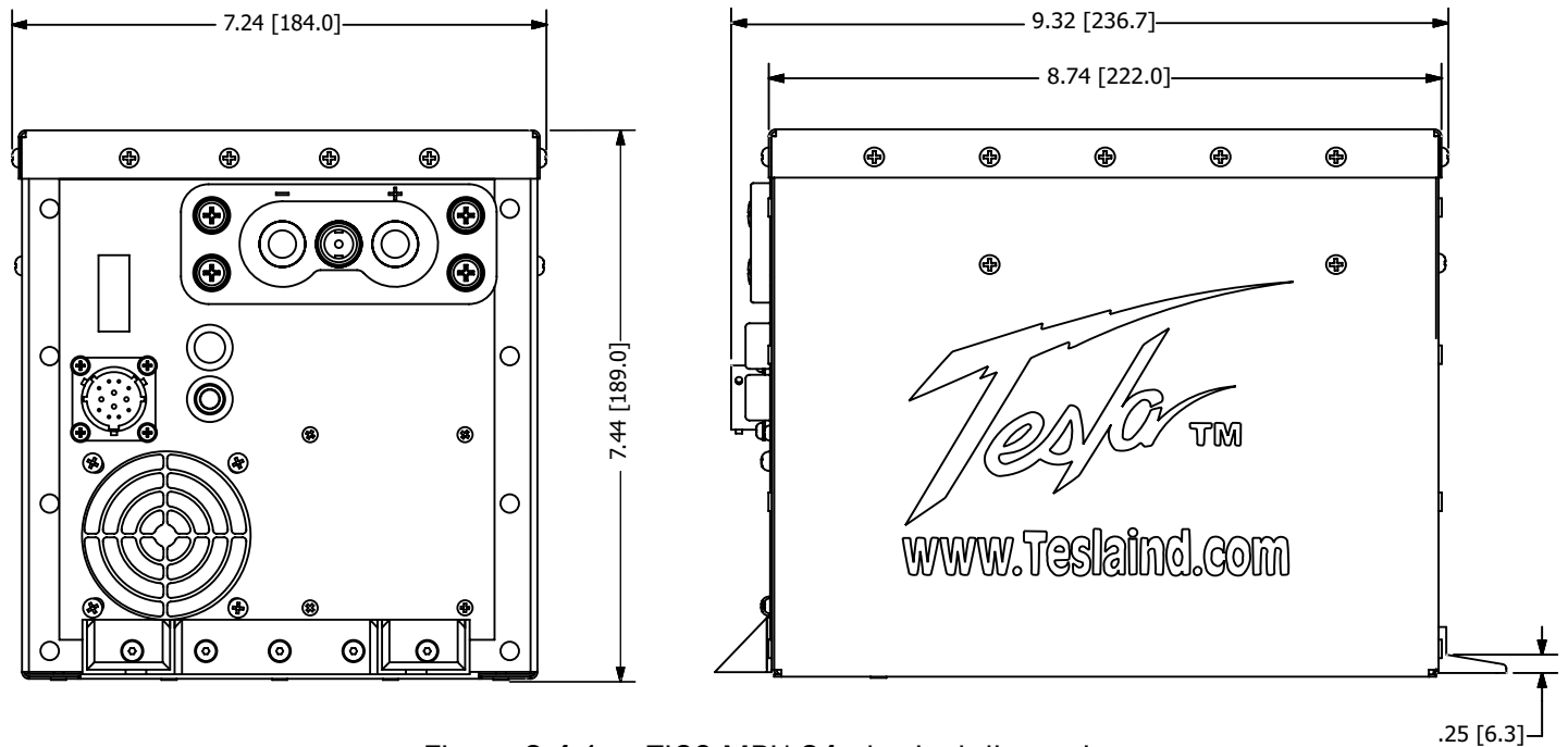
Figure 2.4.1 – TI60 MPU-24 physical dimensions
