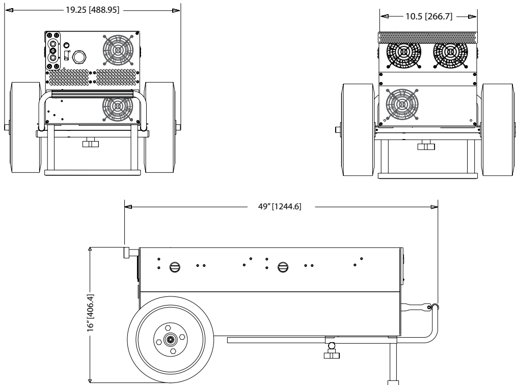
Figure 2.5.1 – TI4200 GPU-24-PFC physical dimensions
