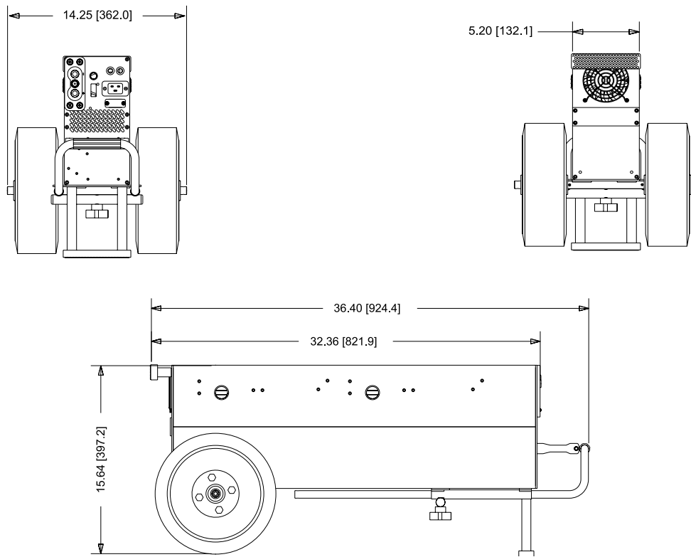
Figure 2.5.1 – TI3000 GPU-24-UNV physical dimensions
