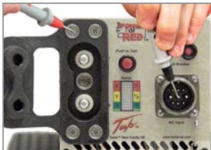
4. Move the positive probe to the fastener screw on the dc receptacle. Multimeter should read less than 1\Omega .
