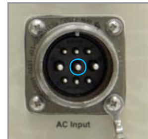
The ground post of the ac input is the middle prong (outlined in blue)
