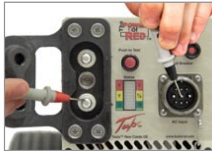
2. Place the negative probe on the ac ground post of the ac input and the positive probe to the dc positive post. Multimeter should read greater than 10\text{ M}\Omega .
