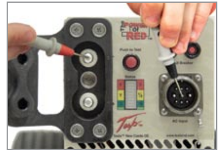
3. Move the positive probe to the dc negative post. Multimeter should read greater than 10\text{ M}\Omega .
