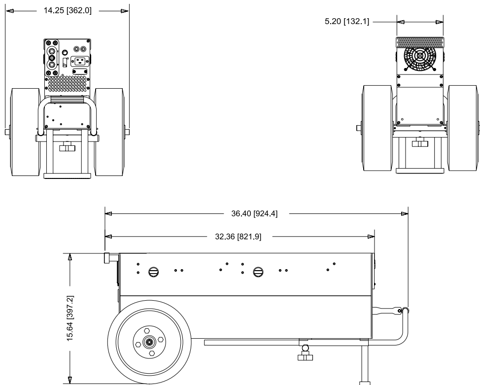
Figure 2.5.1 – TI1590 GPU-12 physical dimensions
