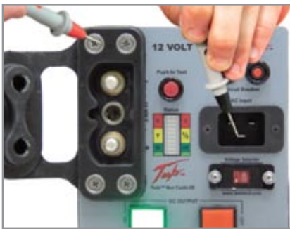
4. Move the positive probe to the fastener screw on the dc Receptacle. Multimeter should read less than 1Ω.
