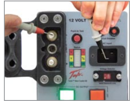
3. Move the positive probe to the dc negative post. Multimeter should read greater than 10 MΩ.
