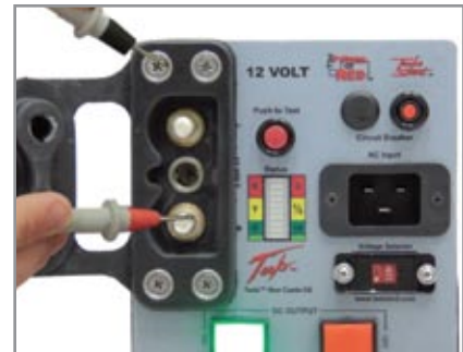
3. Place the negative probe to the fastener screw on the dc receptacle. Move the positive probe to the dc positive post. Multimeter should read 0 Volts.
