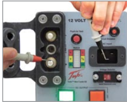
2. Place the negative probe on the ac ground post and the positive probe to the dc positive post. Multimeter should read greater than 10 MΩ.
